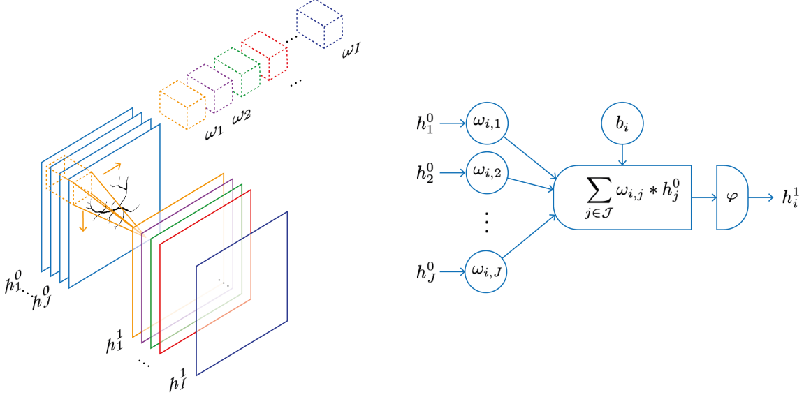
Fig 4 One layer of a convolutional neural network (CNN). ( Left ) The input, consisting of J channels \{h_1^0, \dots, h_J^0\} , is convolved with the I filters \omega_i , then the nonlinearity \varphi is applied and biases b_i added (not shown) to give the output in I channels, \{h_1^1, \dots, h_I^1\} . ( Right ) In analogy with Fig. 3 for the fully connected network, the i^{\text{th}} output channel of a CNN takes an input h^0 \in \mathbb{R}^{m \times m \times J} and computes an output h^1 \in \mathbb{R}^{m \times m \times I} according to Eq. (33).
