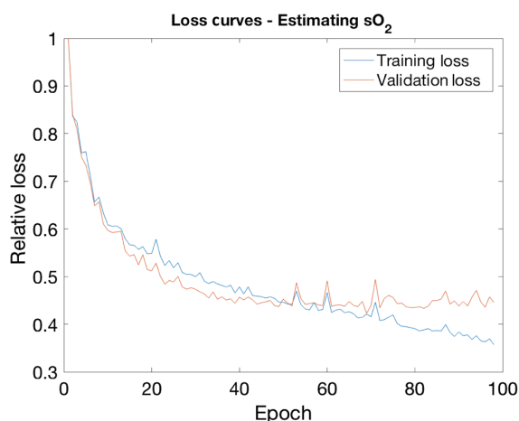
Fig. 4 Relative loss curves ( \epsilon_A ) for the sO_2 estimating network.
