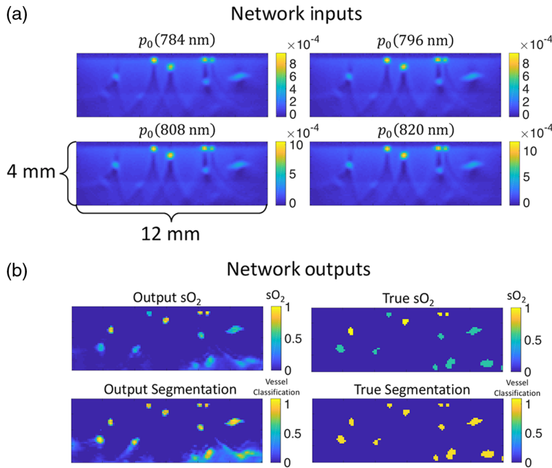
Fig. 3 (a) 2-D slices of 3-D p_0 images simulated at four wavelengths from a single tissue model used as an input for networks A and B . (b) The corresponding 2-D slices of the 3-D outputs of the networks and the ground truths for this example.
